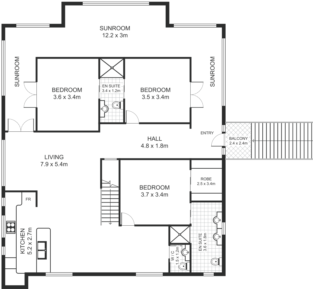
UPPER LEVEL
